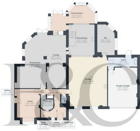
Floor 0
